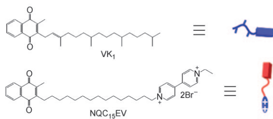
Scheme 1. Structures of VK_1 and molecular wire NQC_{15}EV .
